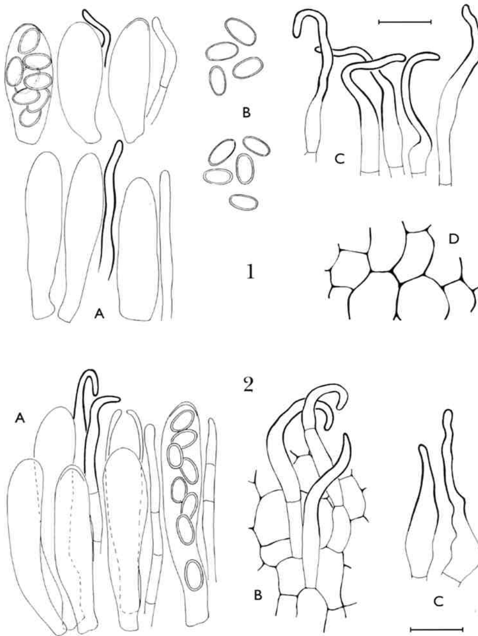
FIGS 1–2. Unguicullella tityrii . FIG. 1. A–D holotype, in Congo red. A asci and two types of paraphyses; B spores; C marginal hairs; D ectal excipulum in surface view. FIG. 2. A–C Richardson 130/97, in Melzer's reagent. A asci and paraphysis; B hairs on medial flanks; C marginal hairs. Scale bar = 10 µm.
